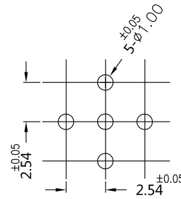
PCB ASSIGNMENT
